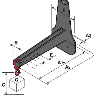
POT: Jib with hook
